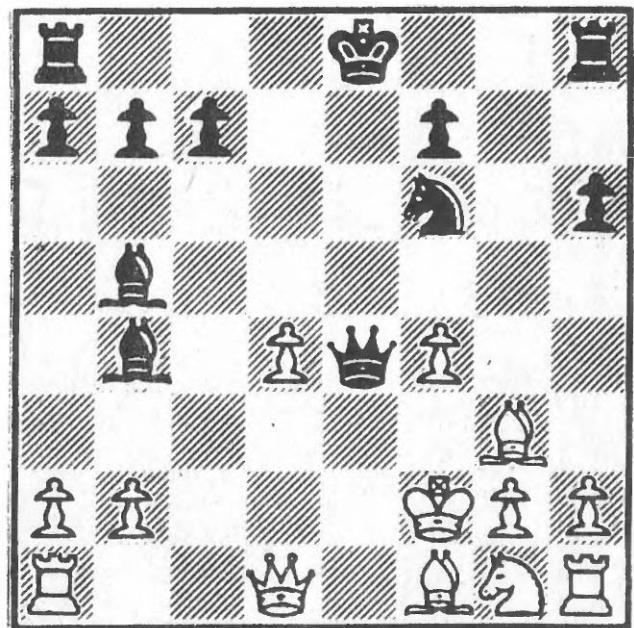
416 After 18 Kf2
